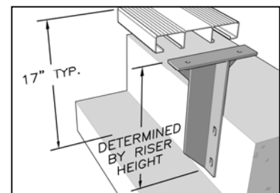
T Bracket
