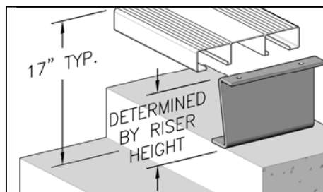
Z Bracket
