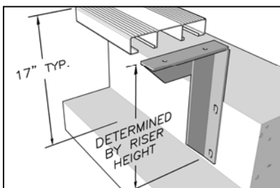
L Bracket
